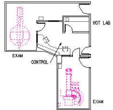
NUCLEAR IMAGING SUITE PLAN
